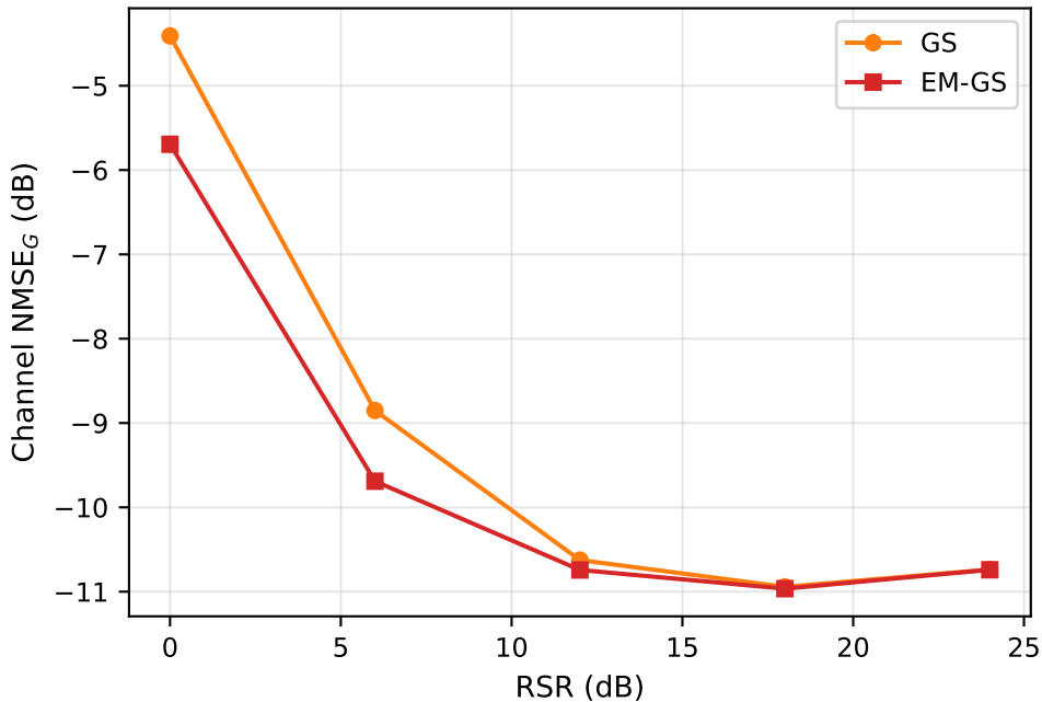
A3: baselines vs reference strength ( N=8 , P=30 , SNR=5 dB)
