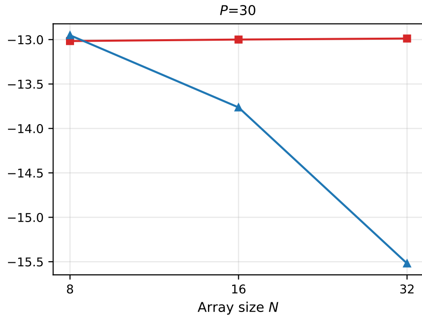
B1: proposed method vs array size ( K=3 , RSR=12 dB)
