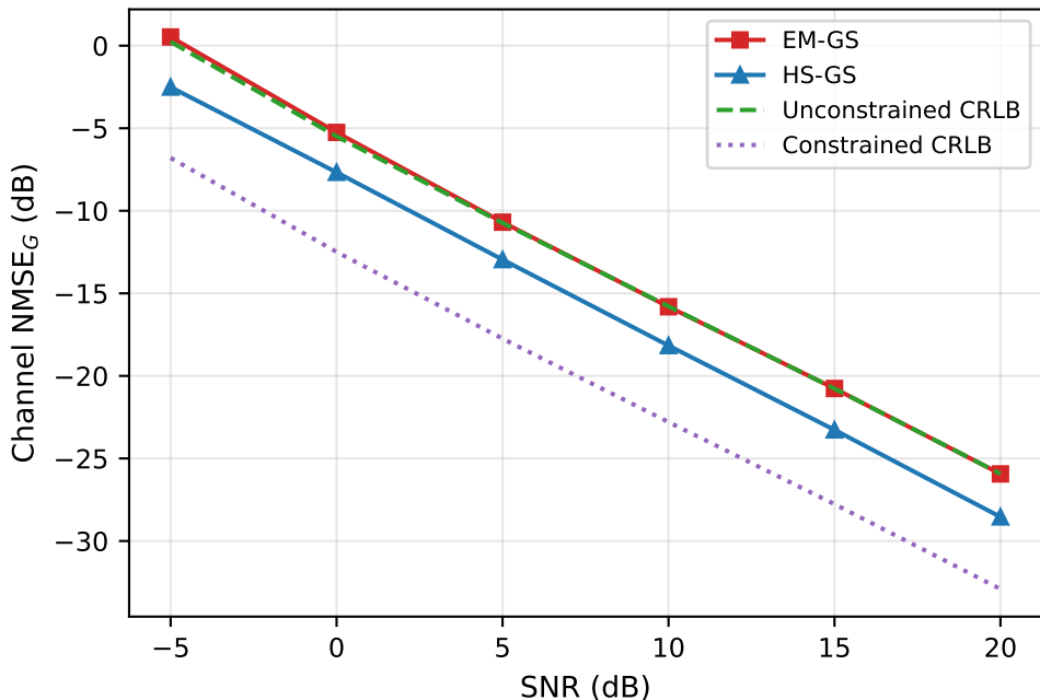
B2: proposed vs SNR ( N=32 , K=3 , P=30 , RSR=12 dB)
