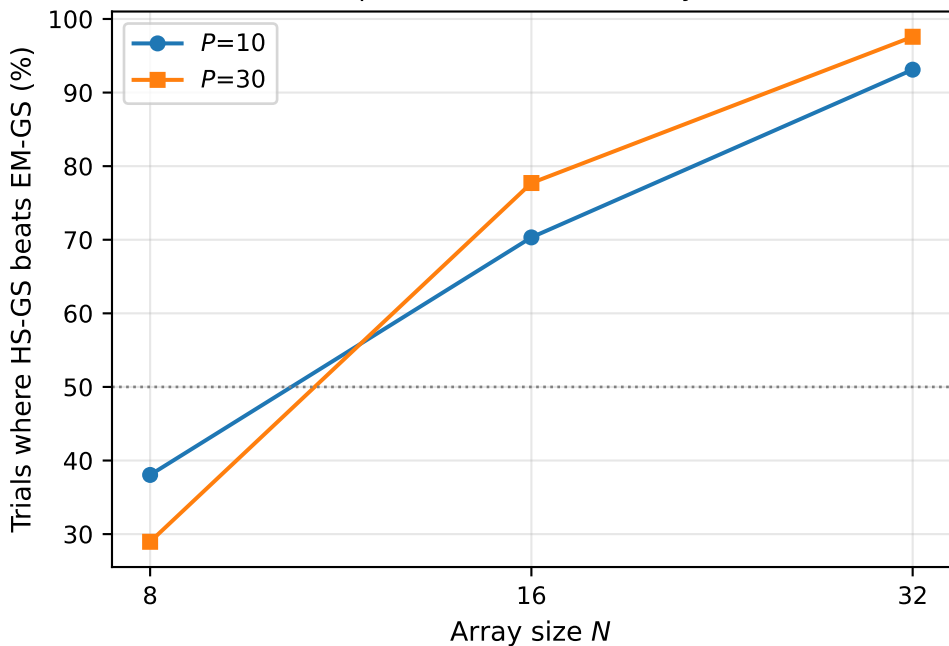
B4: per-trial win rate vs array size
