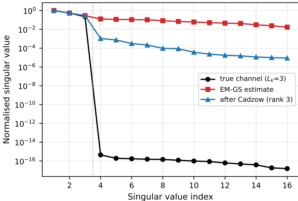
C1: Hankel spectrum, N=32 , one user, SNR=5 dB
