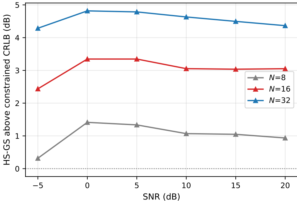
C3: distance from the structured bound ( P=30 )
