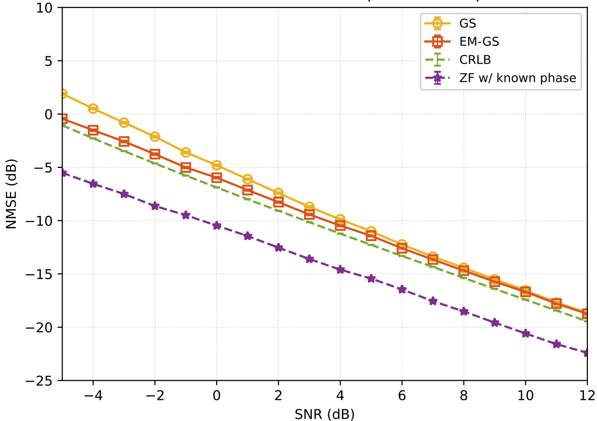
Detection NMSE vs SNR (RSR = 12 dB)
