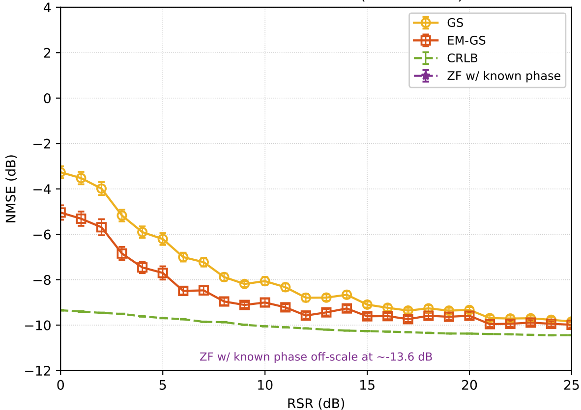
Detection NMSE vs RSR (SNR = 3 dB)
