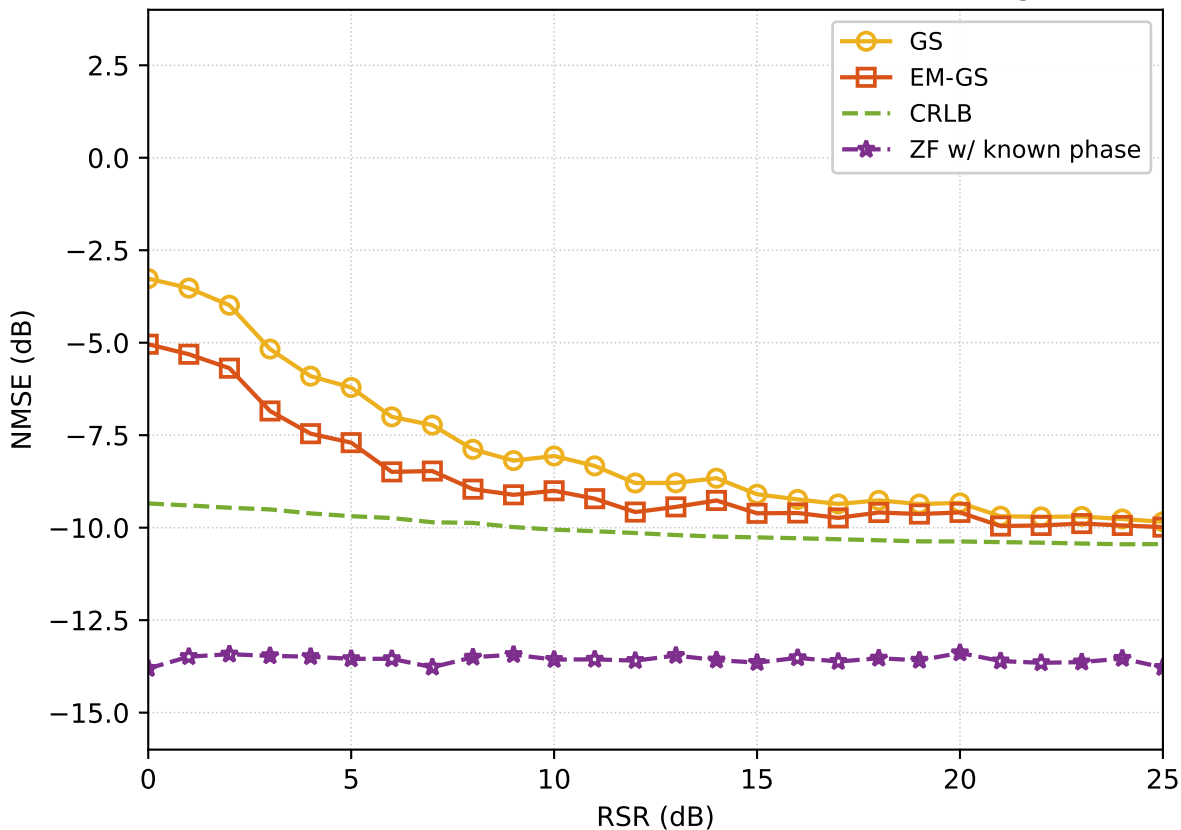
Detection NMSE vs RSR (SNR = 3 dB) -- full range
