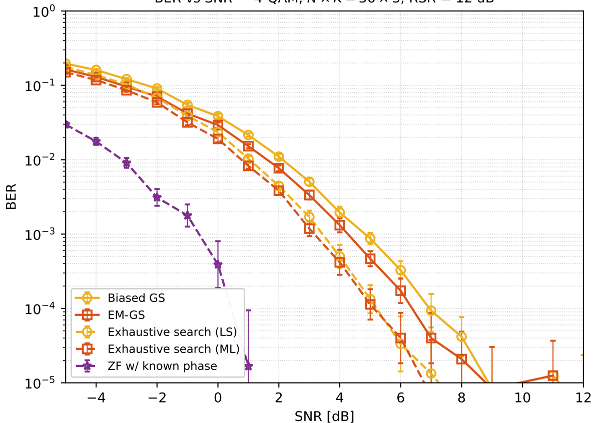
BER vs SNR — 4-QAM, N \times K = 36 \times 3 , RSR = 12 dB
