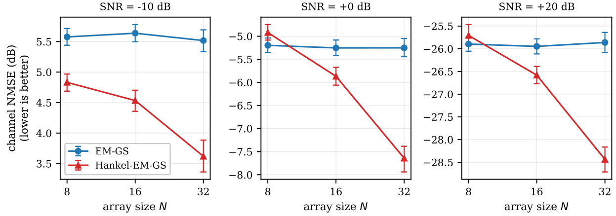
K=3 , P=30 , RSR=12 dB, L_k \sim \mathcal{U}\{3..7\} ; paired trials, identical channel/pilots/noise/initialisation per trial; error bars 95% bootstrap CI
