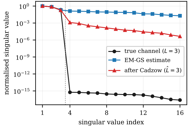
Fig. 4. Normalised Hankel singular values for one channel column, N = 32 , L = 3 , \text{SNR} = 5 dB. The true channel is exactly rank L ; the EM-GS estimate is full rank; Cadzow restores the cliff approximately, to \sim 10^{-3} rather than to machine precision.
