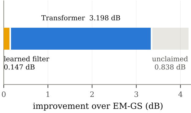
Fig. 1. Attribution of the unrolled estimator's gain over EM-GS at 80k training samples. "Unclaimed" is the remainder of the genie-aided least-squares headroom, which is a reference and not a bound.
