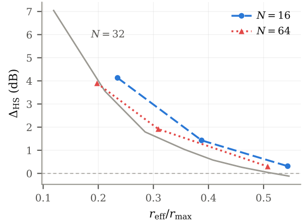
Fig. 2. \Delta_{HS} against \rho = r_{\text{eff}}/r_{\text{max}} for N \in \{16, 32, 64\} . The boundary location is stable across a fourfold change in aperture; the gain magnitude is not, and that residual is unexplained.
