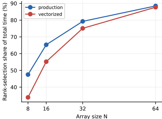
(b) Interleaved estimator; three trials per point
