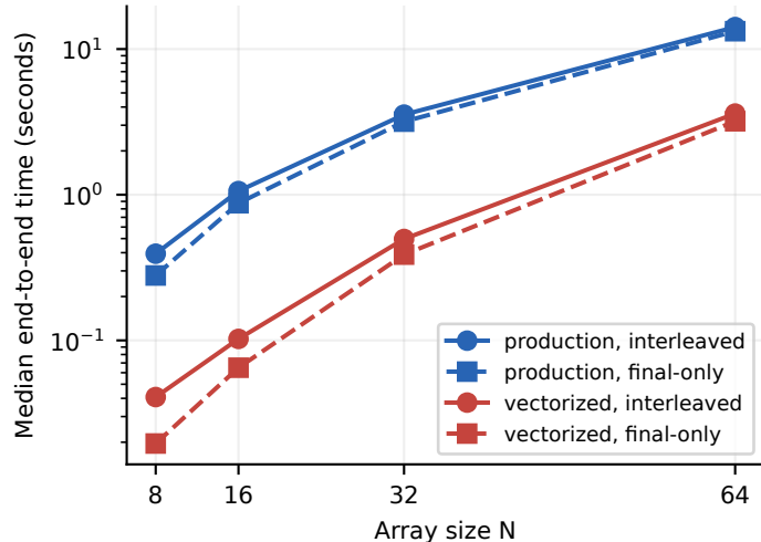
(a) Rank selection included; final-only uses 4 sweeps
