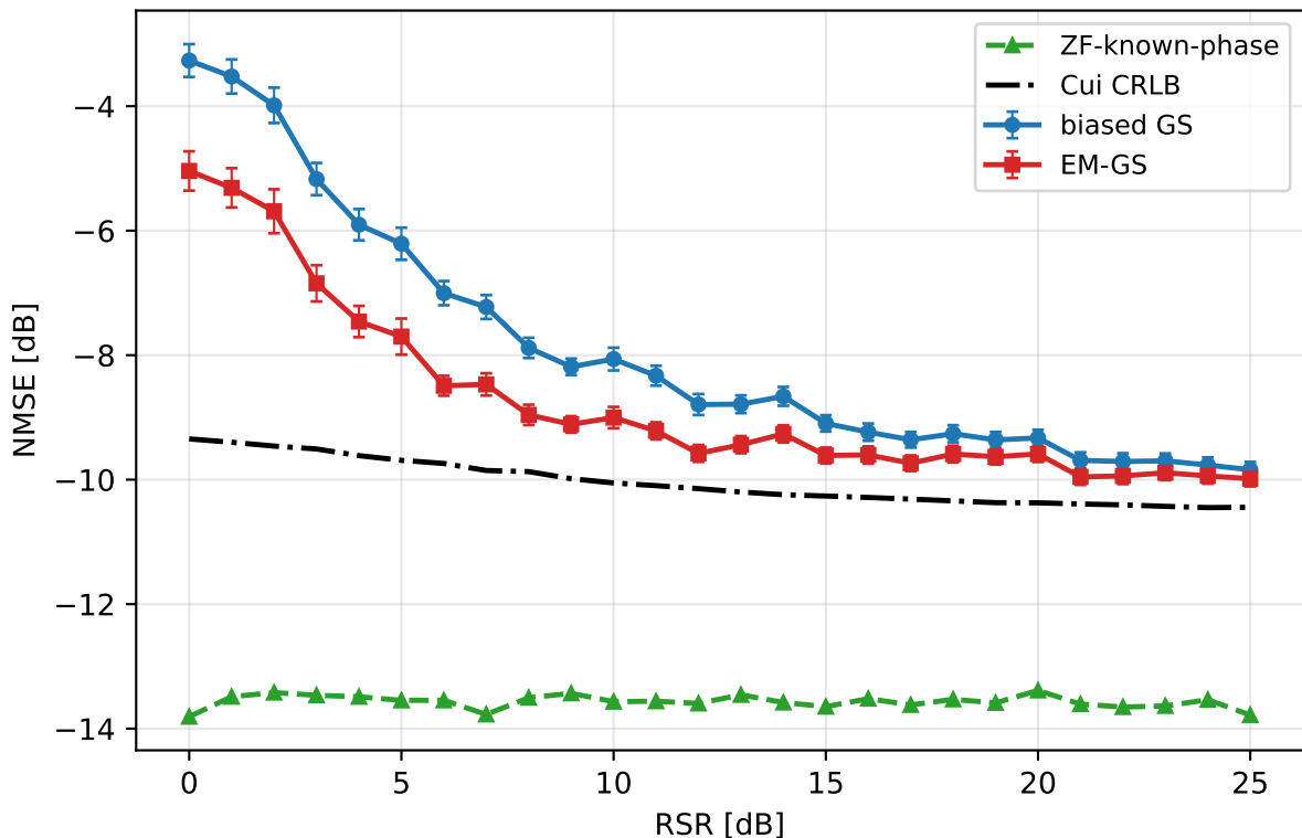
Cui Fig. 6 — detection NMSE vs RSR (Track A), SNR = 3 dB, 16-QAM N=36 K=3 t 0 =50, 500 trials/RSR
