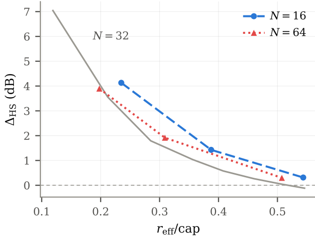
Fig. 2. \Delta_{\text{HS}} against r_{\text{eff}}/\text{cap} . The zero crossing is invariant to within 0.070 across N \in \{16, 32, 64\} ; the gain magnitude is not, with N = 16 exceeding N = 64 by a one-signed mean of 0.493 dB (max. 0.901 dB) at matched ratio. The N = 32 curve is a reference measured at a fixed 5 dB and is not paired with the other two.
