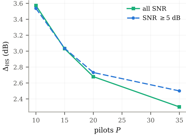
Fig. 4. The structural gain grows as pilots become scarce. Adaptive rank, at the default configuration.
