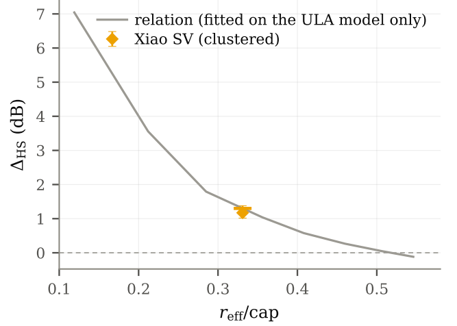
Fig. 3. Predictions registered before measurement, against measurement. The relation is fitted on the ULA model of (2) only; neither channel here was used to fit or tune it.
