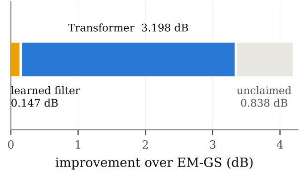
Fig. 1. Where the unrolled estimator's gain over EM-GS comes from, at 80,000 training samples. The remainder is the gap to the genie-aided least-squares reference, which is a reference and not a bound.
