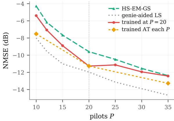
Fig. 3. Pilot efficiency against pilot-count generalization at 5 dB, on identical realizations. The dashed diamonds are separate networks trained at each P ; the solid curve is one network trained at P = 20 .
