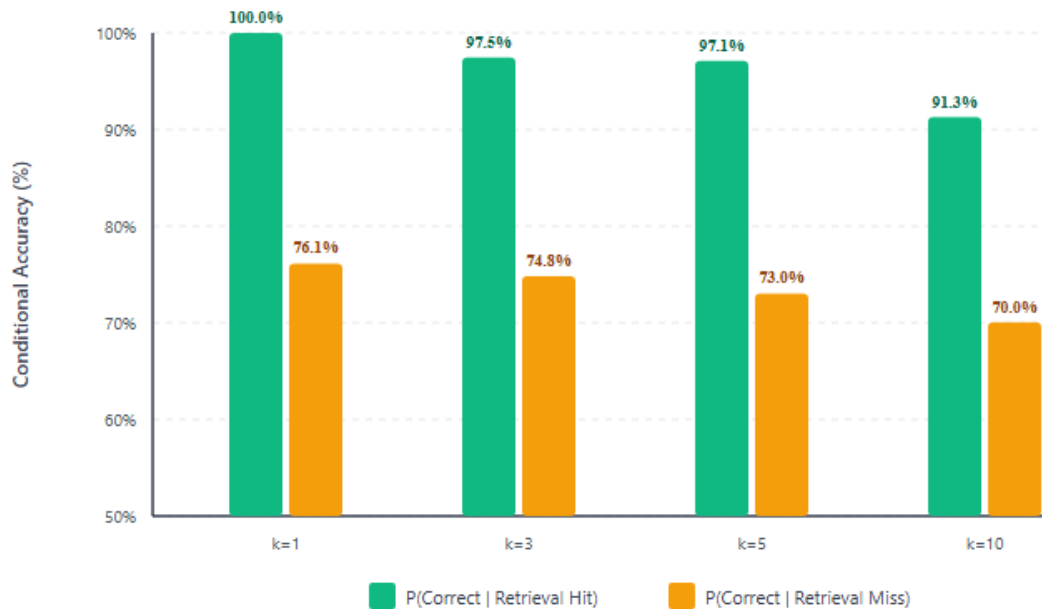
Figure 5: Downstream Attribution Accuracy Conditioned on Retrieval Success
