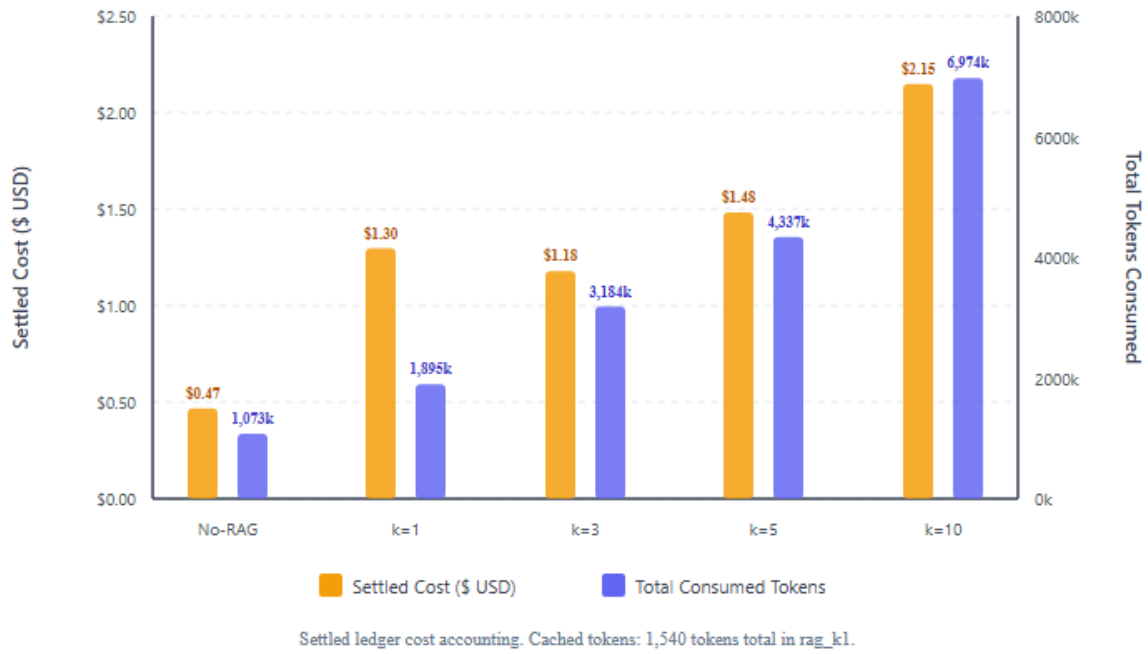
Figure 7: Settled Financial Spend (USD) and Aggregate Token Consumption across Experimental Conditions.
