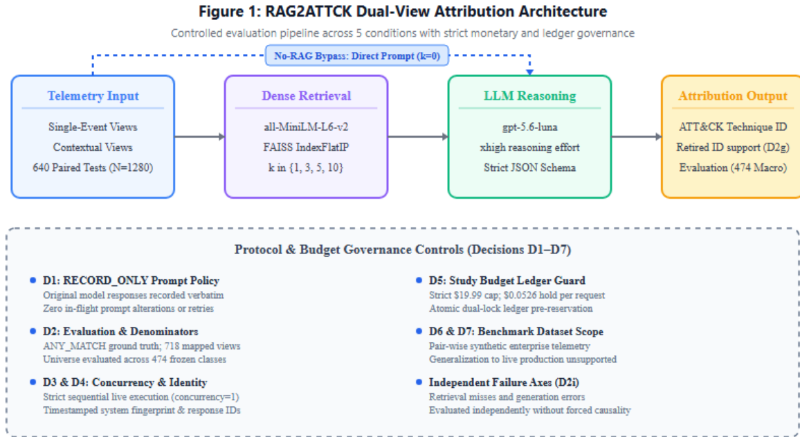
Figure 1: Dual-View Attribution Architecture (CTI Log -> all-MiniLM-L6-v2 -> FAISS -> gpt-5.6-luna xhigh).
