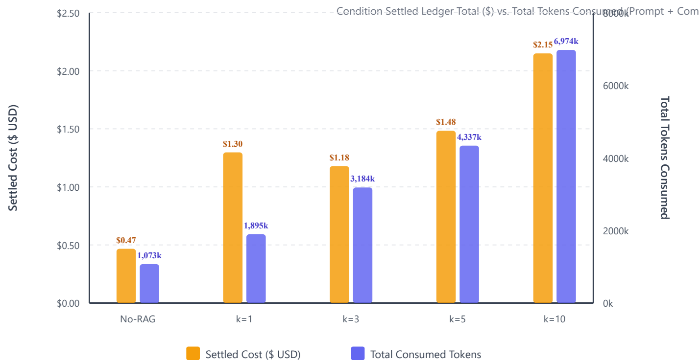
Figure 7: Financial Cost ($) and Token Usage Scaling /
