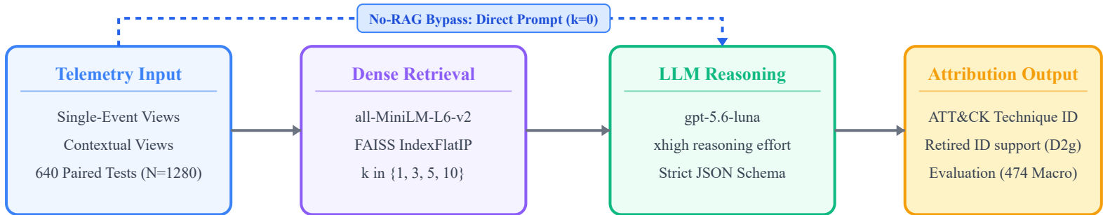
Figure 1: RAG2ATTCK Dual-View Attribution Architecture
