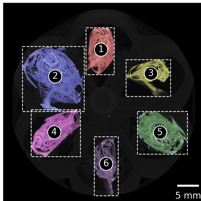
6 detected fish
