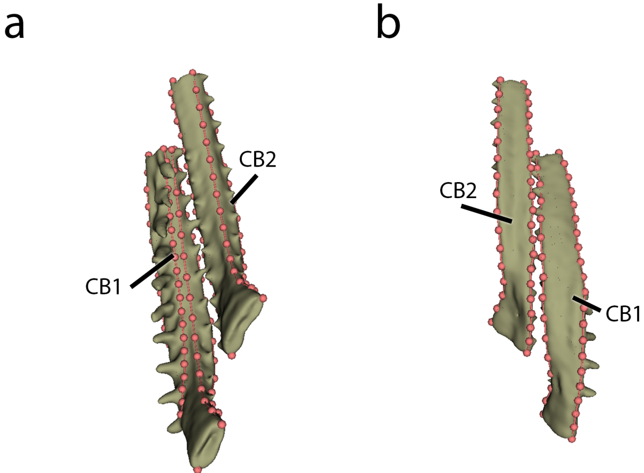
Figure 9: Landmarking shown on dorsal (a) and ventral surfaces (b).
