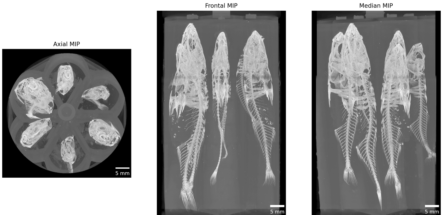
Figure 3: Maximum intensity projections of one acquired dataset along all three cardinal axes.
