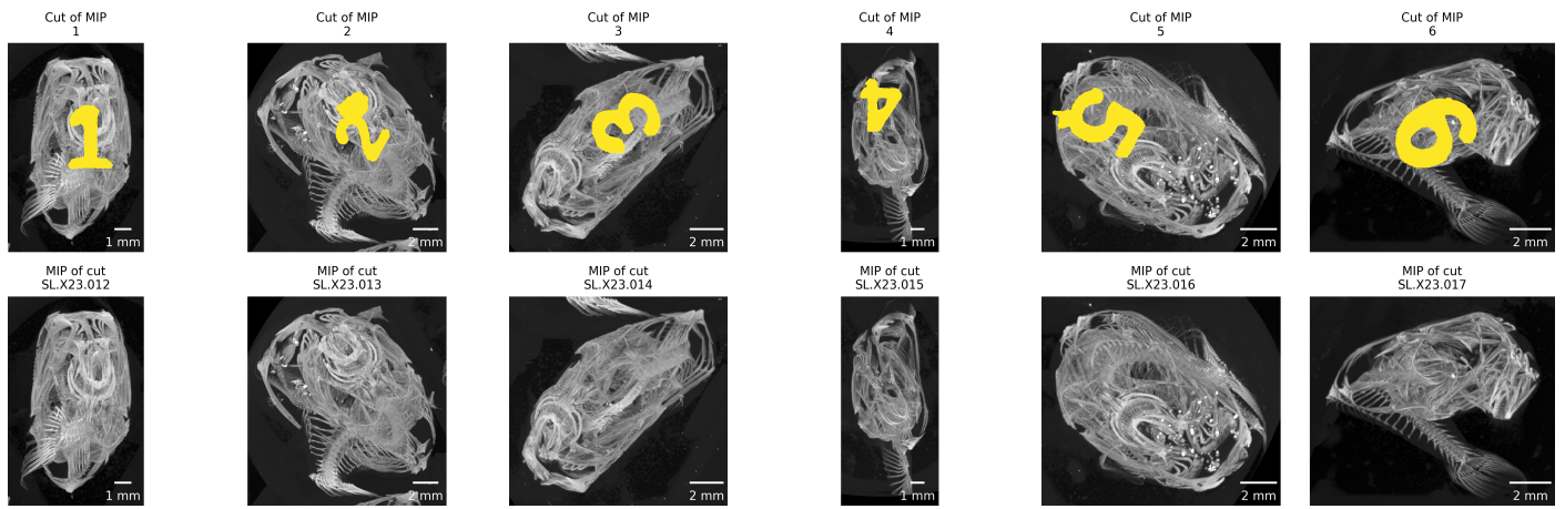
Figure 6: Double-checking crop extent and fish ID. The top row shows the extracted regions from the previously calculated MIP of the full scan, the bottom row shows the MIP images of the extracted regions. Both rows must show exactly the same region.
