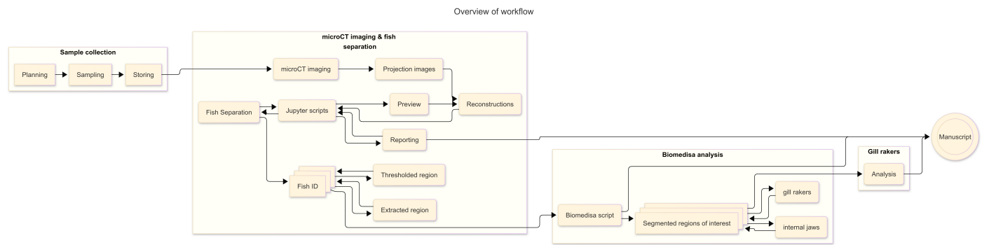
Figure 1: Workflow overview
