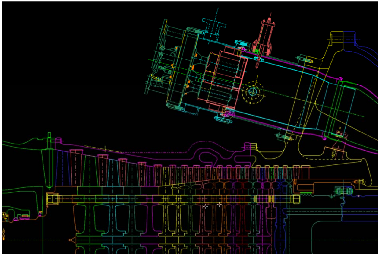
6FA Cross Section
