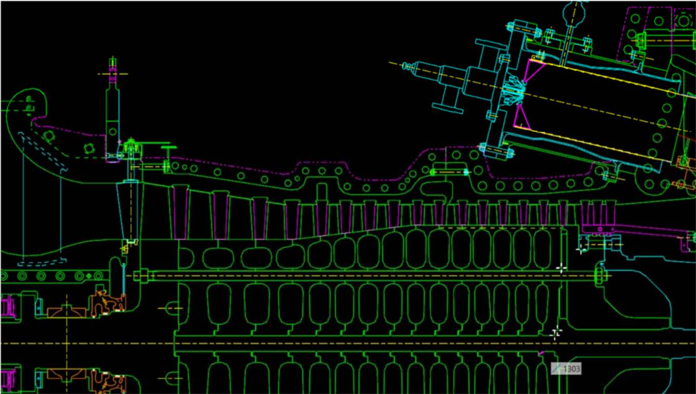
6B Cross Section
