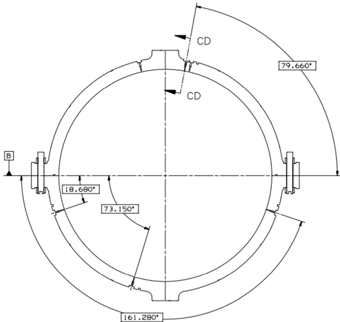
SECTION CC-CC (C7, SH3) R14 ROTOR RIM 6 POINT LOCATIONS
