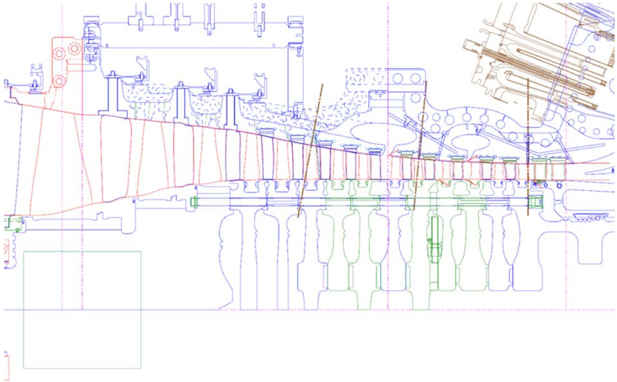
7HA.02-16 Cross Section
