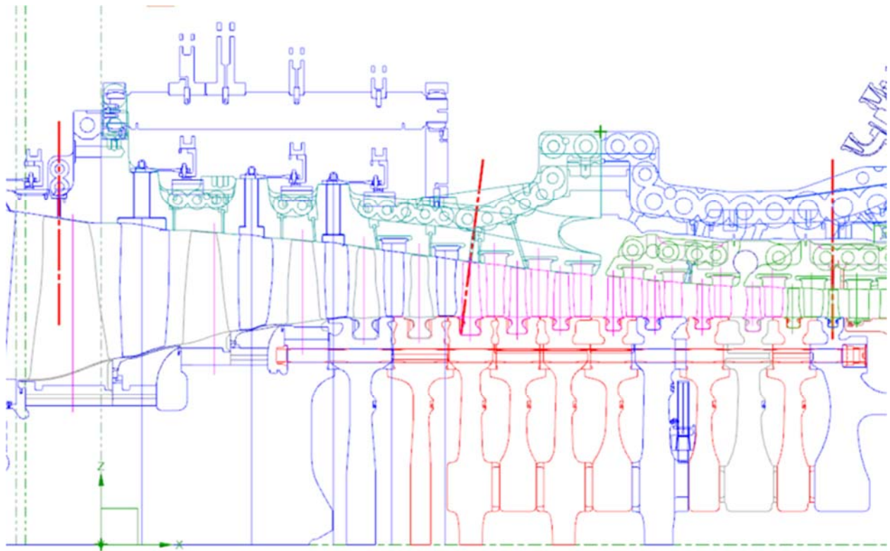
9HA.01 Cross Section
