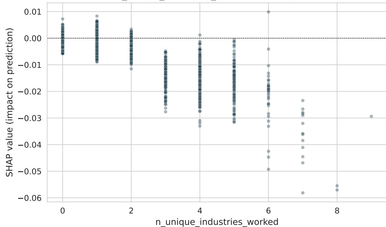
How 'n_unique_industries_worked' affects predictions
