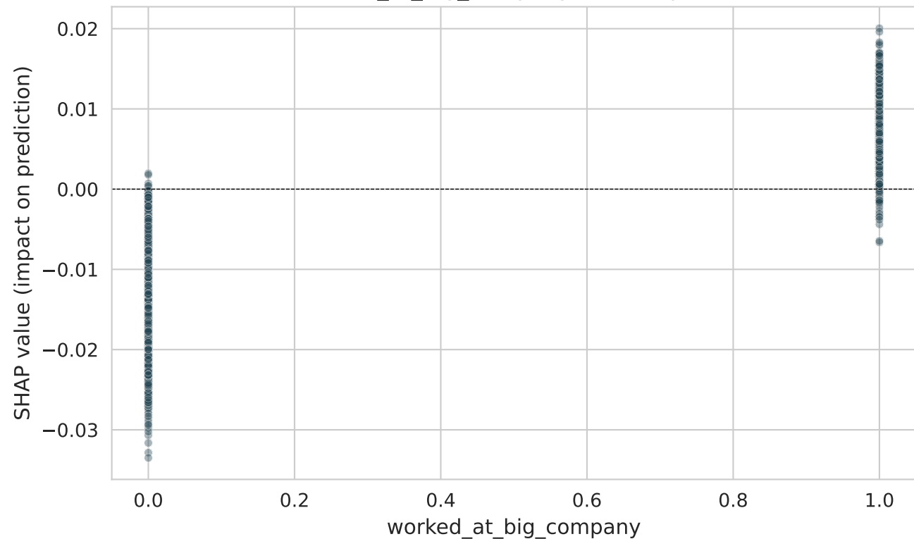
How 'worked_at_big_company' affects predictions
