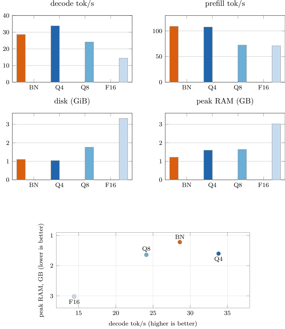
Figure 12: Independent efficiency re-evaluation on one x86 laptop: decode throughput (mean of five repeats at a common four-thread point), on-disk size (exact), and peak resident memory (a single sample at eight threads, essentially thread-independent). BN (orange) is the BitNet b1.58 2B4T I2_S checkpoint; Q4, Q8, and F16 (blues) are Qwen2.5-1.5B-Instruct at Q4_K_M, Q8_0, and FP16. The bottom panel plots decode throughput against peak memory: BitNet and Q4 share the Pareto frontier, while Q8 and F16 are dominated on both axes.
