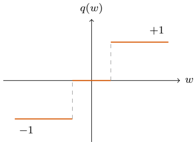
(a) forward pass: the quantizer q(w)
