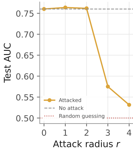
Credit Default
