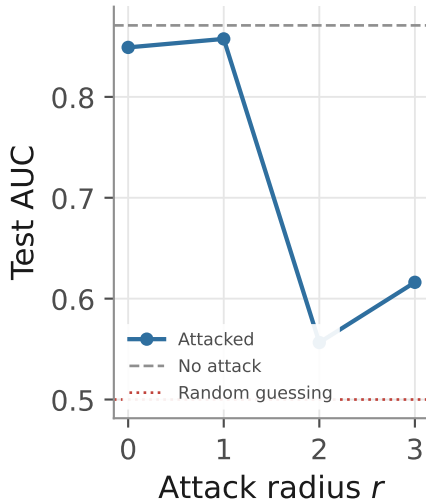
Heart Disease
