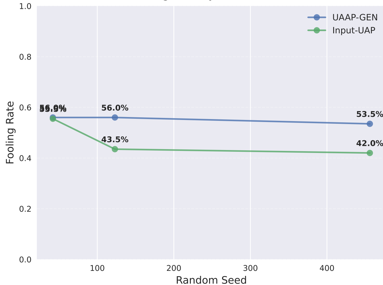
Fooling Rate by Seed (MNIST)
