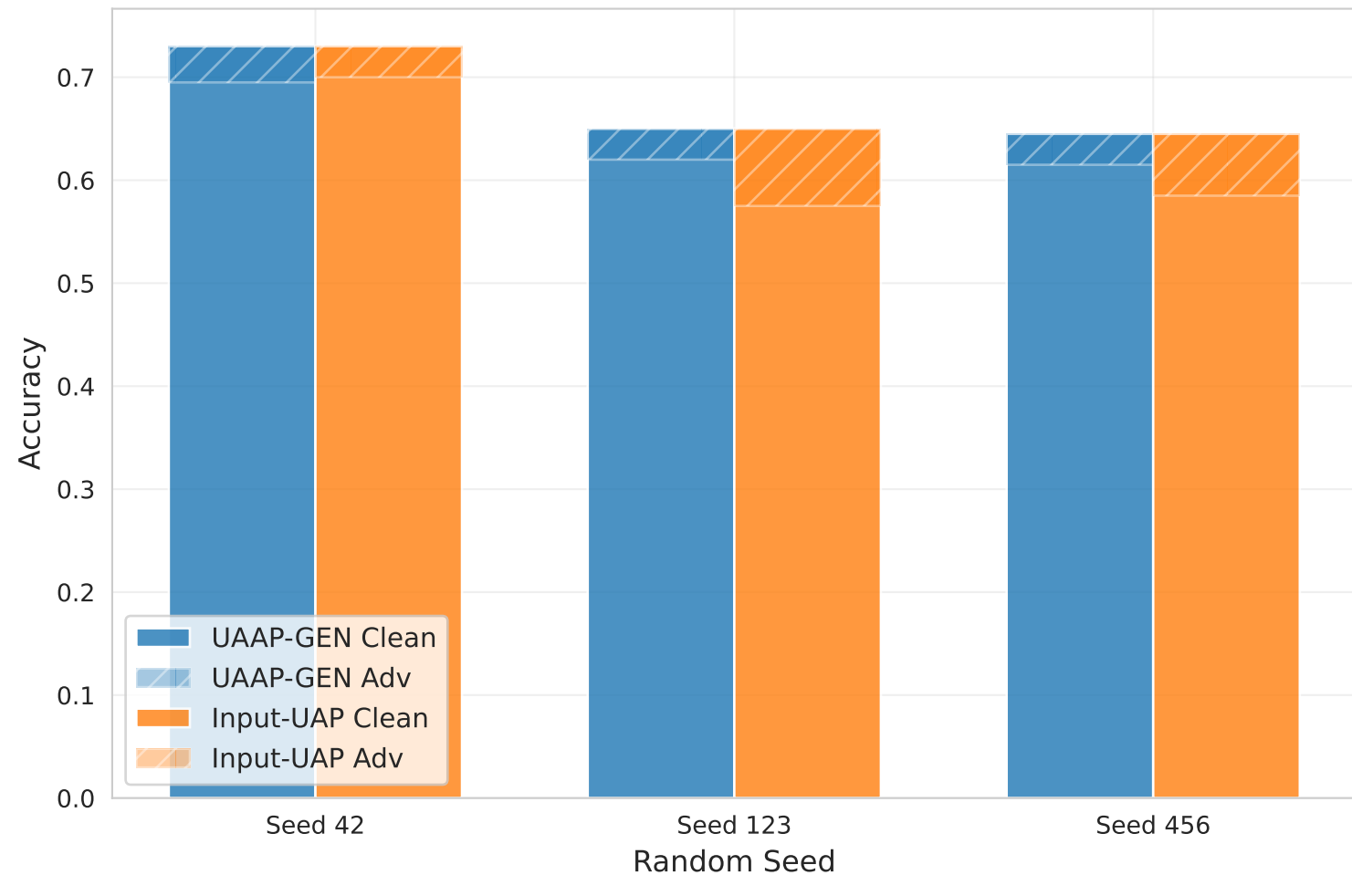
Clean vs Adversarial Accuracy (MNIST, 2-Layer ViT)
