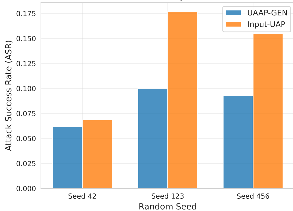
Attack Success Rate Comparison (MNIST, 2-Layer ViT)
