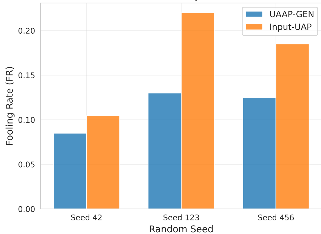
Fooling Rate Comparison (MNIST, 2-Layer ViT)
