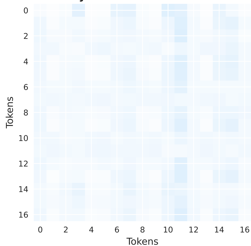
Layer 2 - Clean Attention
