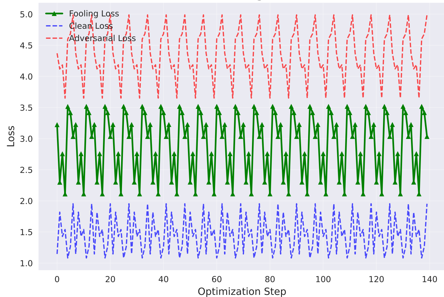
UAAP Generation: Fooling Loss Maximization
