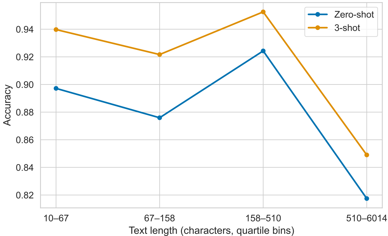
Accuracy by text length
