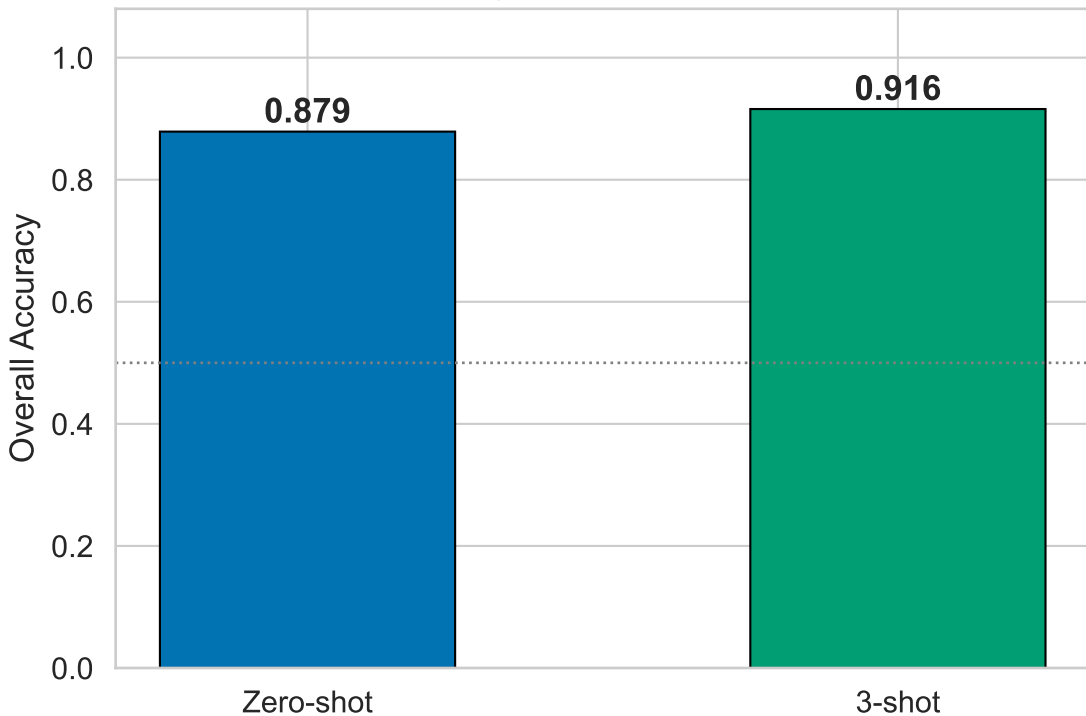
Final Score: Zero-shot vs Few-shot gemma-3-4b-it
