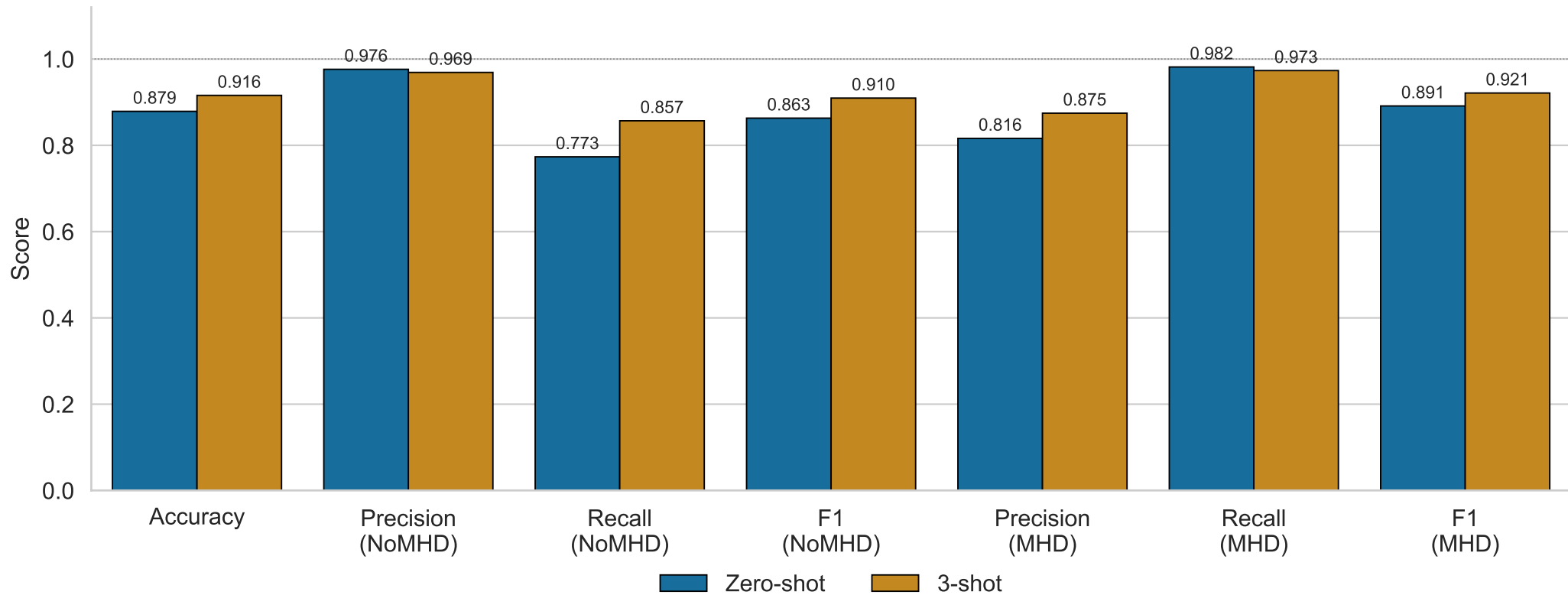
Zero-shot vs Few-shot performance — gemma-3-4b-it
