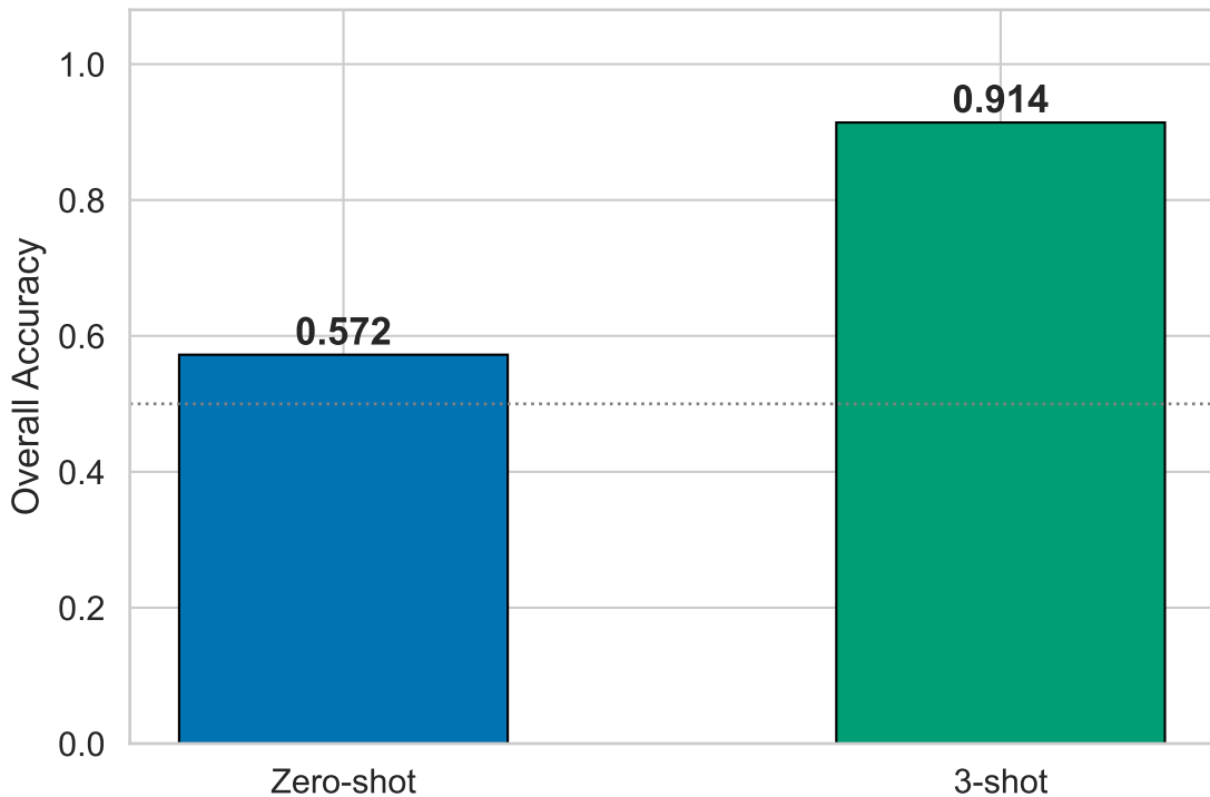
Final Score: Zero-shot vs Few-shot llama-3.2-3b-instruct
