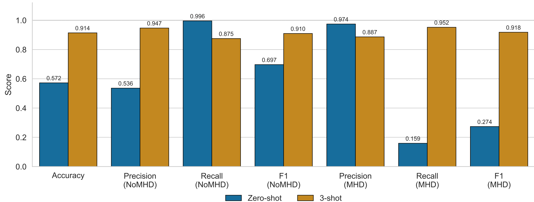
Zero-shot vs Few-shot performance — llama-3.2-3b-instruct
