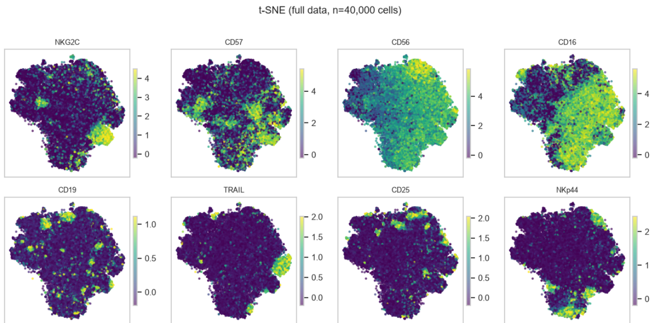
Figure A4. The same markers and cells on the saved t-SNE map. NKG2C/CD57 expression can guide follow-up of a memory-like NK phenotype, but expression gradients alone do not validate a functional adaptive population or label individual cells as CMV-infected. The plots' "full data" titles refer to the full balanced analysis sample, not all 261,593 available NK cells.
