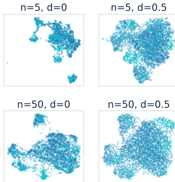
Figure A2. Four settings from the original UMAP grid. Rows contrast 5 with 50 neighbours; columns contrast min\_dist=0 with 0.5. Smaller min\_dist permits tighter packing; n\_neighbors changes the graph's neighbourhood scale. Parameter-induced islands are not independently established cell types.
