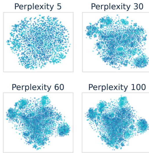
Figure A1. Selected original t-SNE sweep panels with enlarged parameter labels: perplexity 5, 30, 60 and 100. Same fixed 5,000 cells, 29 PCs and seed 42. Blue/cyan denote CMV-negative/positive donor labels. Trustworthiness at 60 is only slightly above the values at 50 and 100.
