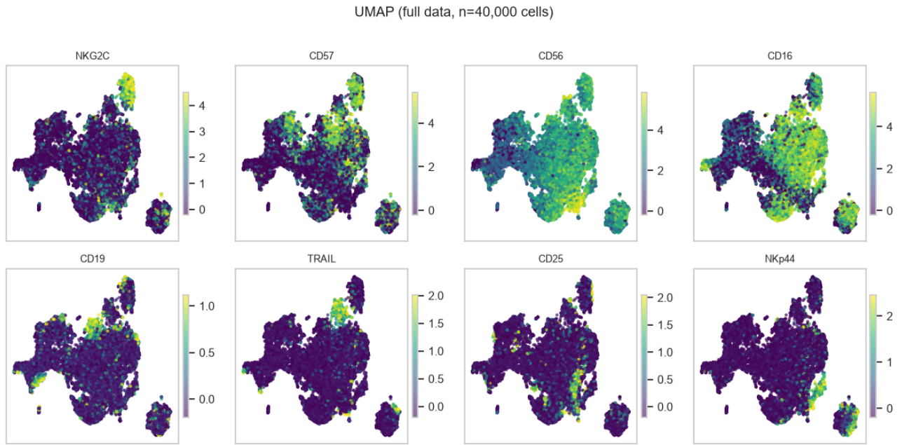
Figure A3. Original UMAP marker overlays from notebook cell 41 (counting from 1), on the balanced 40,000-cell sample. Each panel colours the same points by a different arcsinh-transformed marker; colour limits are clipped at that marker's 1st/99th percentiles. Numerical scales therefore differ between markers.
