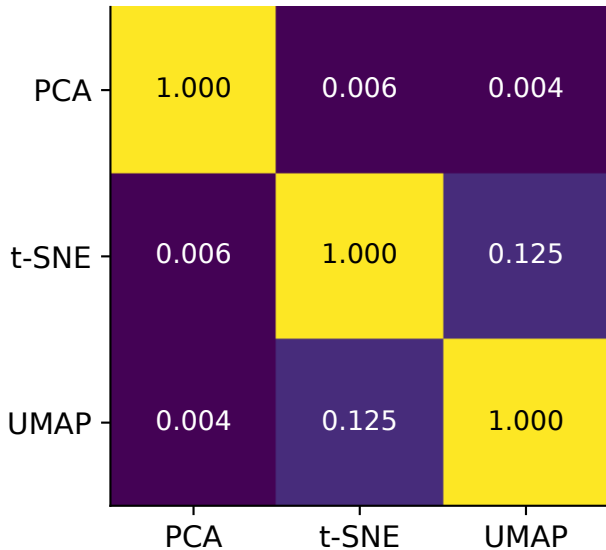
Shared neighbours, k=15
