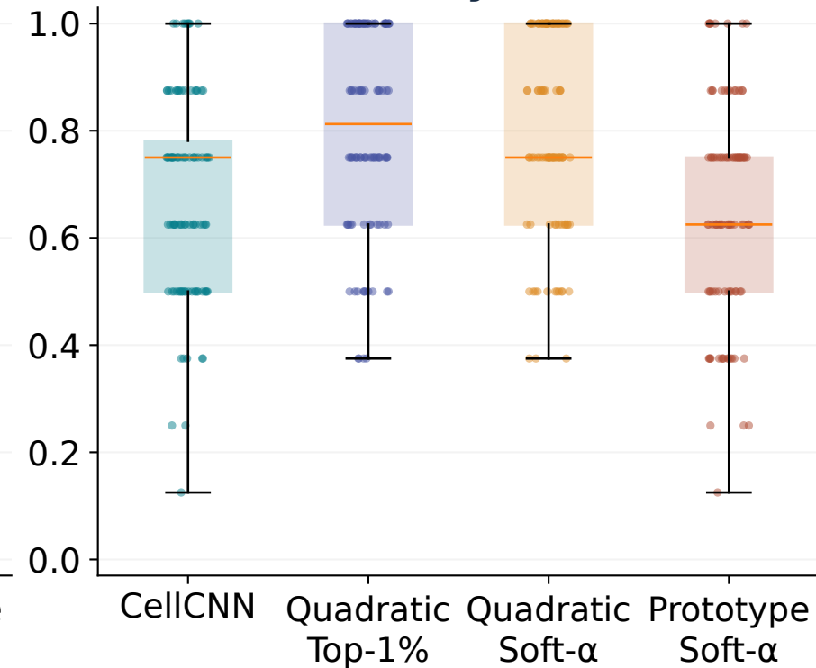
Balanced accuracy (threshold 0.5)
