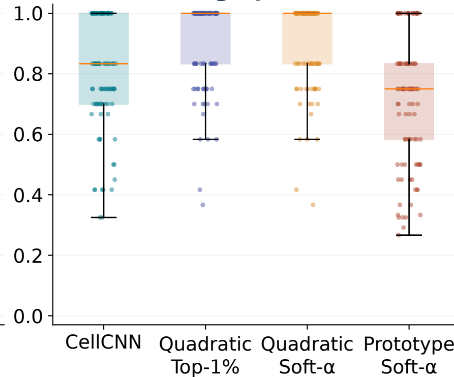
Average precision
