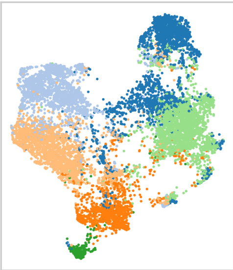
K-Means: 6 Cluster
