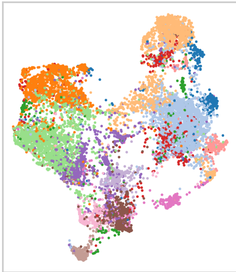
Ward: 14 Cluster
