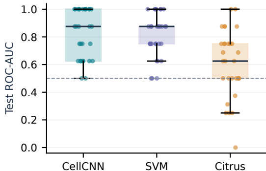
A Classification performance
