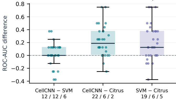
B Paired differences on the same splits
