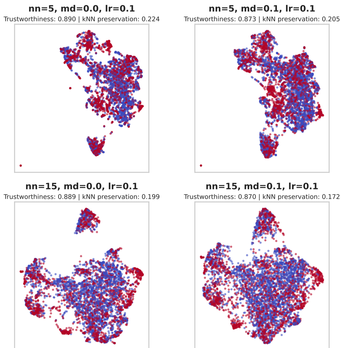
Figure S5: UMAP parameter examples at learning rate 0.1, first part, left half of the saved grid. Splitting the original vector figure preserves readable parameter labels. All numerical results are in Table S9.
