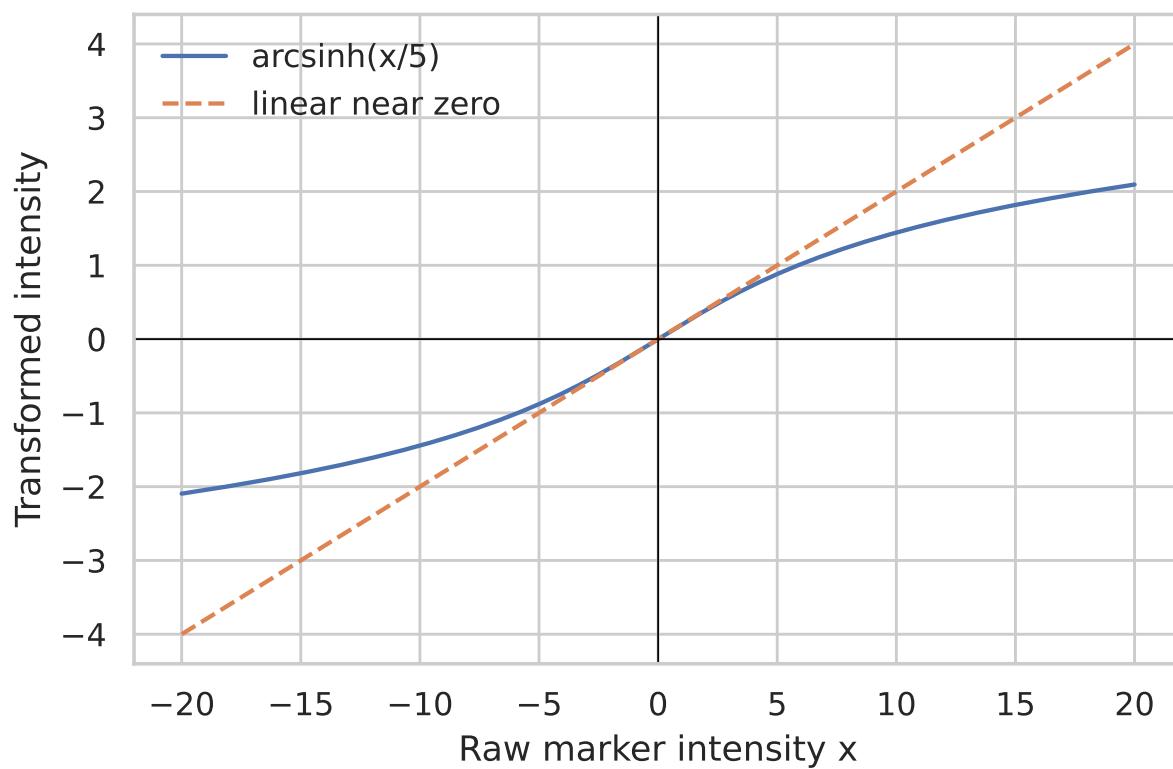
Figure S2: Analytical transformation \text{asinh}(x/5) and its local linear approximation x/5 . This curve illustrates compression of large intensities and retention of negative values. It is not an empirical marker distribution or a cofactor-optimisation result.
