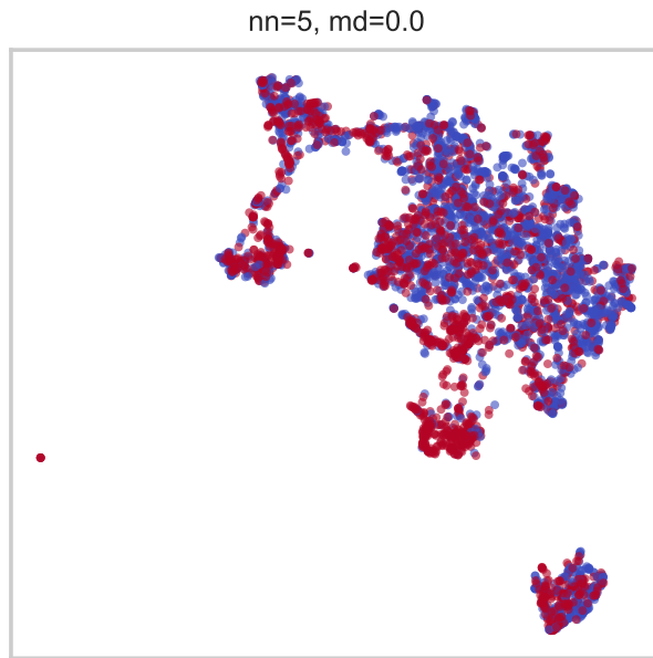
Figure A2. Four settings from the original UMAP grid. Rows contrast 5 with 50 neighbours; columns contrast min_dist=0 with 0.5. Smaller min_dist permits tighter packing; n_neighbors changes the graph's neighbourhood scale. Parameter-induced islands are not independently established cell types.
