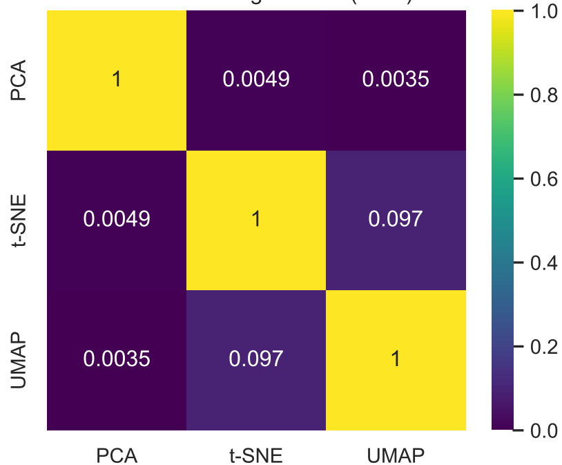
Pairwise kNN agreement (k=15)
